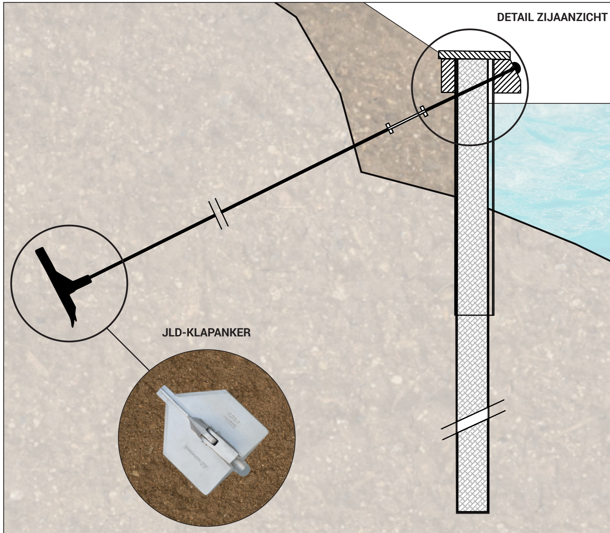
DETAIL VERANKERING DAMWAND : SPANWARTEL+ BOLKOPBOUT
