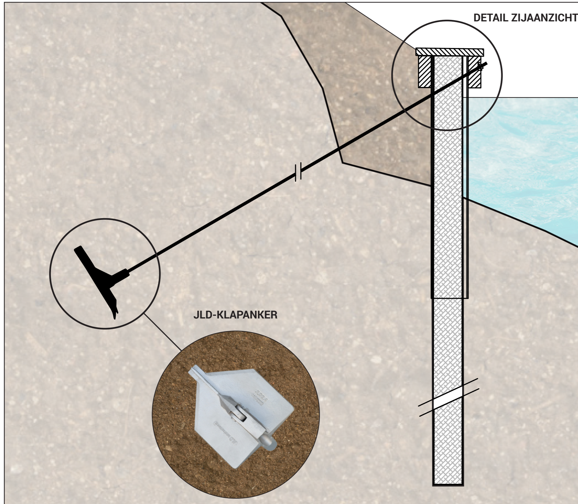
DETAIL VERANKERING DAMWAND : ECONOMIC
