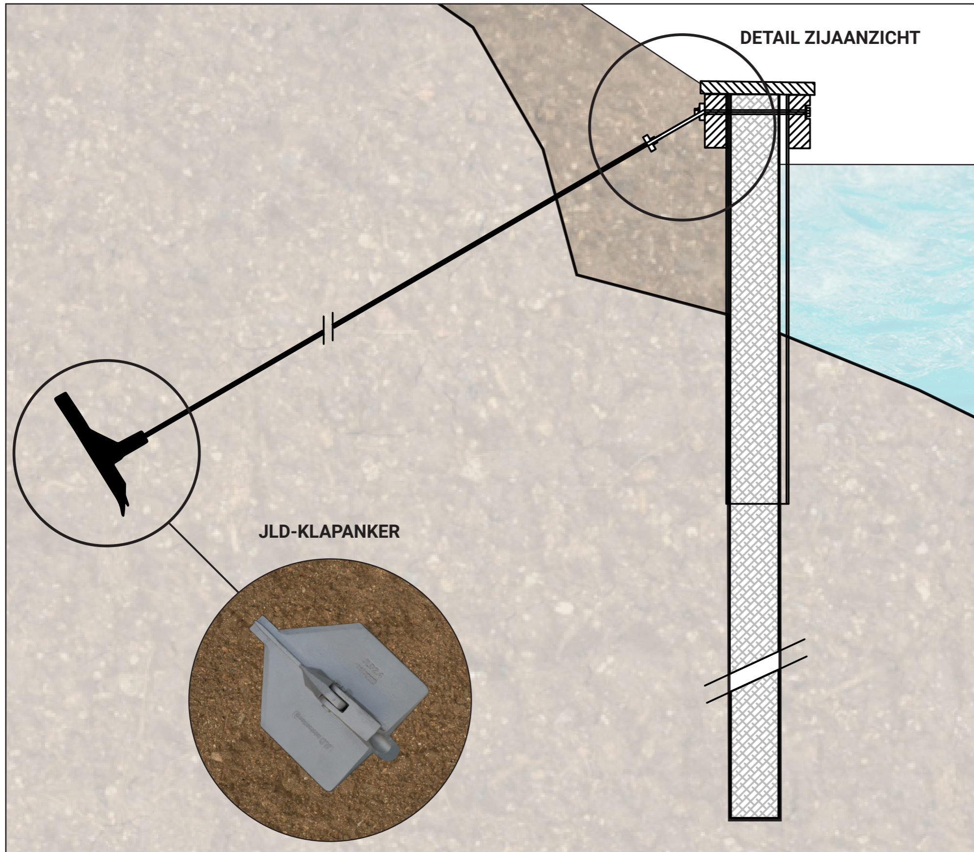
DETAIL VERANKERING DAMWAND : ANKERGORDINGKOPPELING + SLOTBOUT
